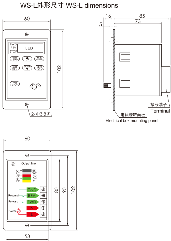
数显面板调速器 Digital panel speed controller
