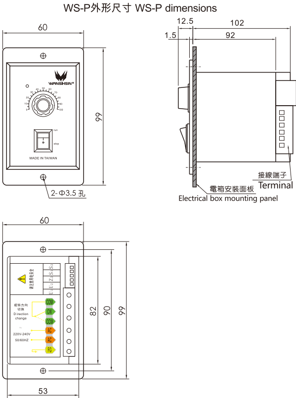
面板式调速器 Panel speed controller
